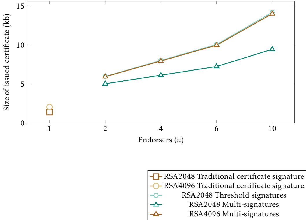
Figure 5.2: Number of Endorsers and size of issued certificates.
