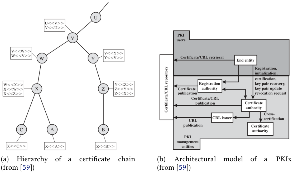
Figure 2.1: Hierarchy of a PKI certificate chain (left) and Architectural model of a PKIx (right)
