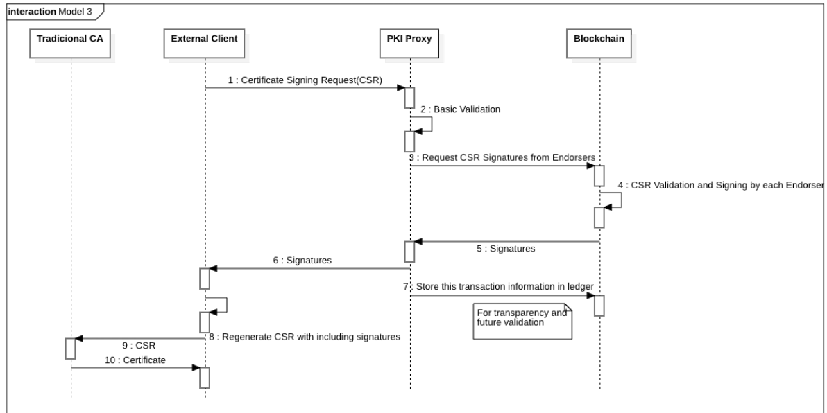
Figure 3.4: CSR Model Sequence Diagram
