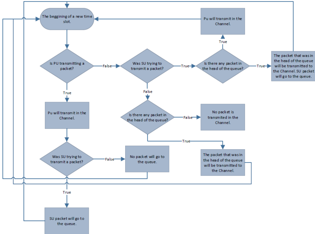
Figure 3.1: Simulation Algorithm.
