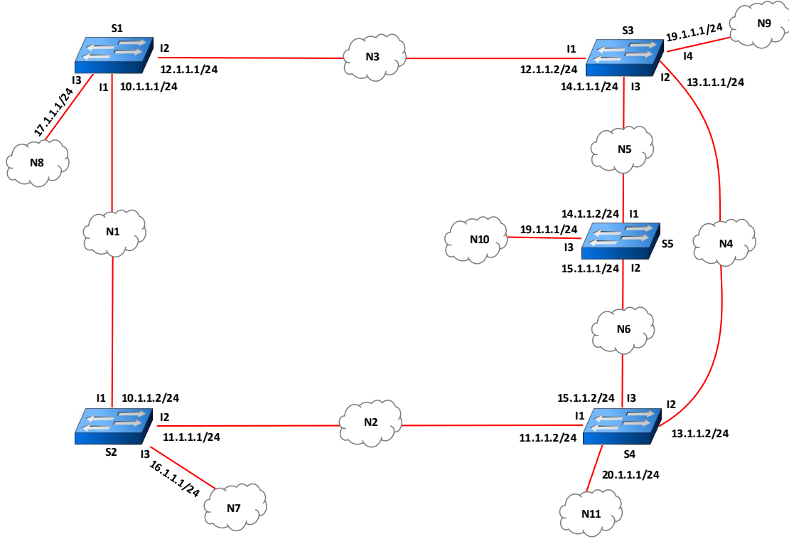
Figure 5.1: The production network topology
