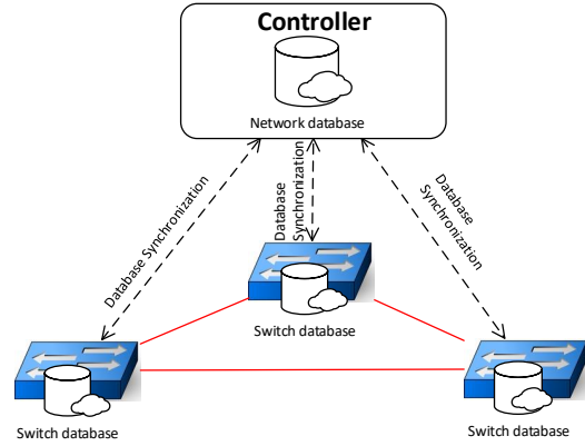
Figure 3.2: DBCP network.
