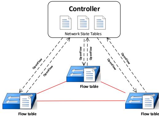
Figure 3.1: OpenFlow network.
