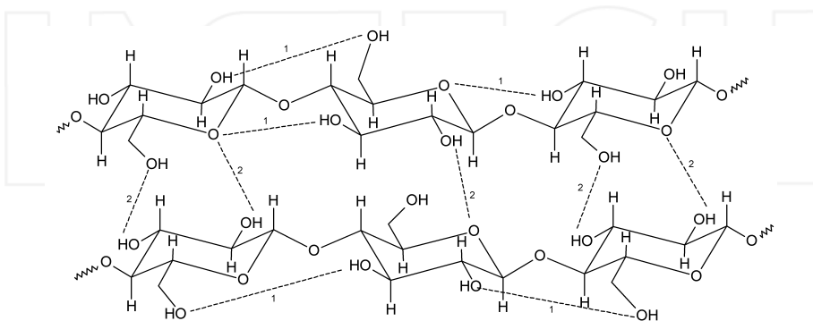
Figure 1. The structure and intra- (1) and interchain (2) hydrogen bonding pattern in cellulose.
