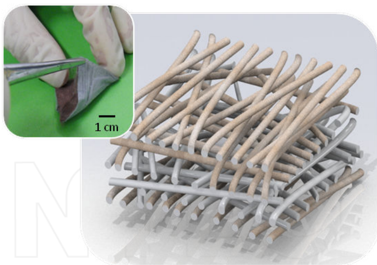
Figure 4. Schematic and macroscopic image of the bio-battery developed by our group. It consists in a cellulose acetate membrane, produced by electrospinning, covered with metallic layers to form the electrodes.
