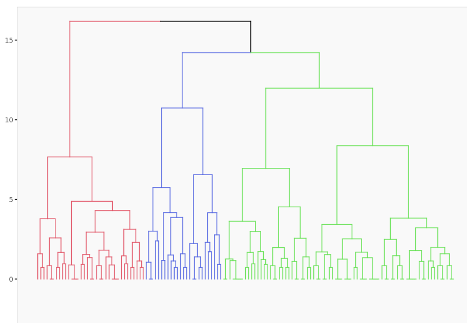
Graph 20: Segmentation –Dendrogram
