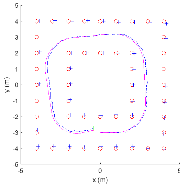
Figure 6.3: Scenario 1 - Simulation result with the MHE method, XY plane
