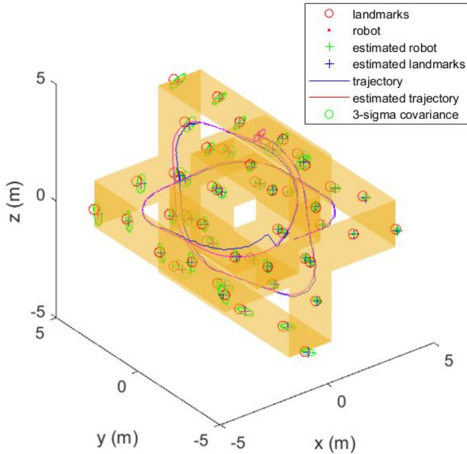
Figure 8.6: Scenario 2 - EKF-based SLAM method
