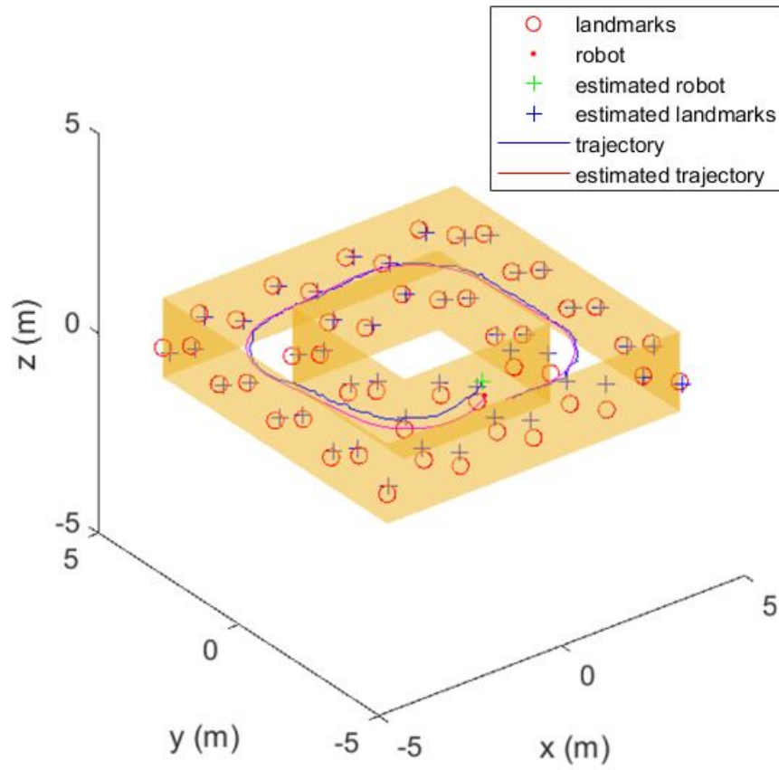
Figure 6.2: Scenario 1 - Simulation result with the MHE method
