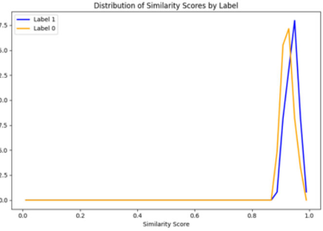
Figure 55: SFR-Embedding-Mistral - Distribution of Similarity Score by Labels
