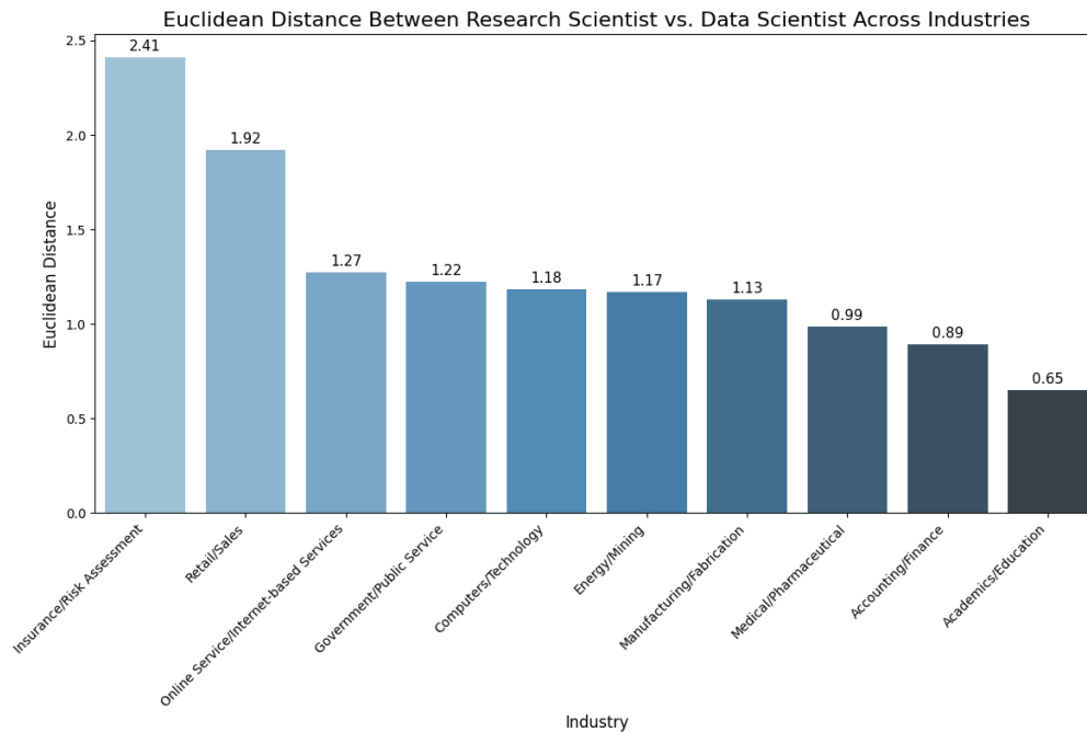
Figure 32: Euclidean distance Across Industries for Research Scientist and Data Scientist
