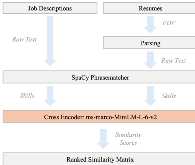
Figure 56: Cross-Encoder Workflow: This diagram illustrates the Cross-Encoder architecture's workflow. Unlike the Bi-Encoder, the Cross-Encoder jointly processes job descriptions and résumés, generating a similarity score in a single step.
