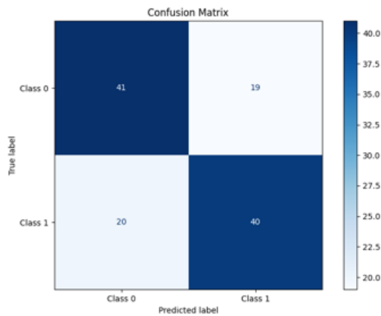
Figure 48: Confusion-Matrix - all-mpnet-base-v2
