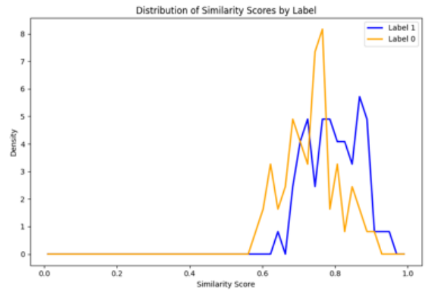
Figure 51: all-MiniLM-L6-v2- Distribution of Similarity Score by Labels
