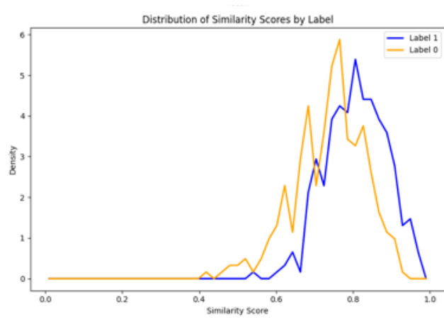
Figure 58: Distribution of Similarity Score by Labels - Bi-Encoder
