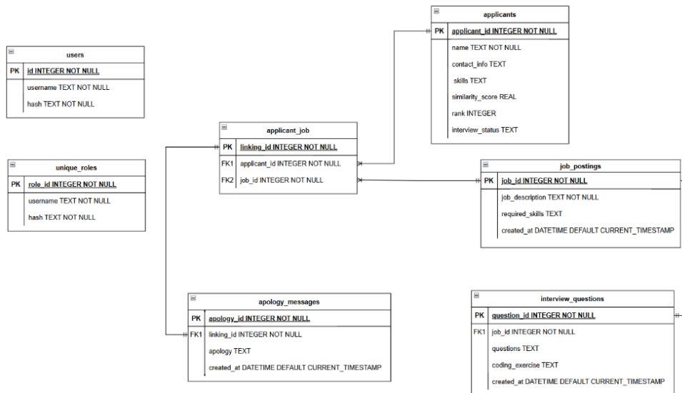
Figure 18: The ER diagram illustrates the database schema for the Skillmatch.ai: Key tables include users, applicants, job_postings, and interview_questions, with relationships managed through the applicant_job linking table. The schema ensures modularity, allowing efficient storage, querying, and management of user data, job postings, and role-specific features.
