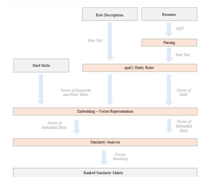
Figure 62: Skills Based Model Steps. First, skills from résumés in PDF format are extracted with the spaCy Entity Ruler. Role Vectors are created combining extract skills from role descriptions and hard skills from O*NET. We then embed the skills using a semantic embedding model (in our case MPNET) before we conduct a similarity analysis with cosine similarity.
