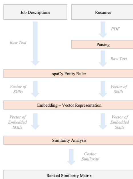
Figure 6: Matching Model Pipeline: The pipeline starts with two inputs, résumés in PDF format and job descriptions in raw text. First, we extract raw text from pdf formatted résumés. Next, we use the spaCy Entity Ruler to extract skills from the two inputs. We then embed the skills using a semantic embedding model (in our case MPNET) before we conduct a similarity analysis with cosine similarity.
