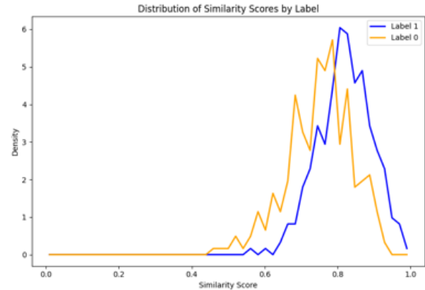
Figure 39: Skill-by-Skills - Distribution of Similarity Score by Labels
