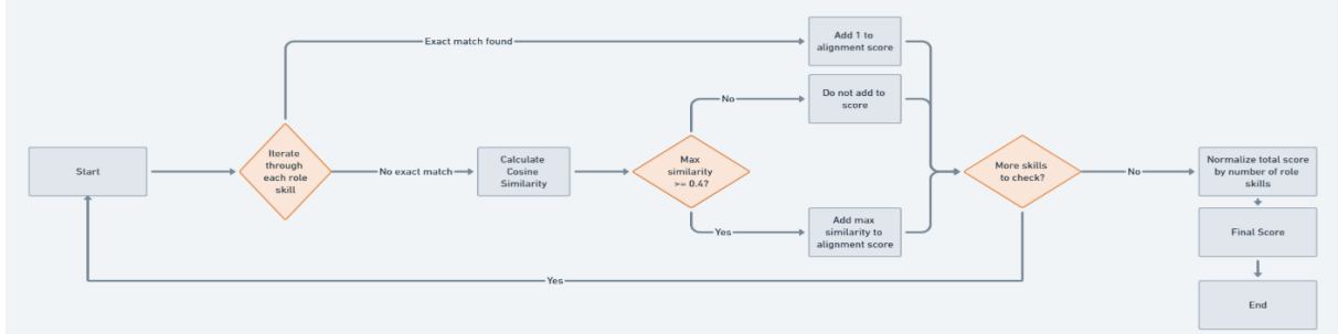
Figure 14: The Scoring Approach: This approach is based on calculating a score based on exact matches and cosine similarity.
