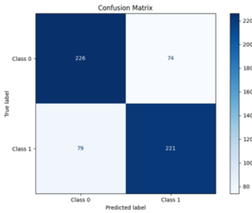
Figure 40: Confusion Matrix - Threshold 0.3
