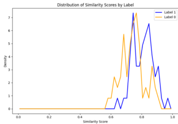
Figure 49: all-mpnet-base-v2 - Distribution of Similarity Score by Labels
