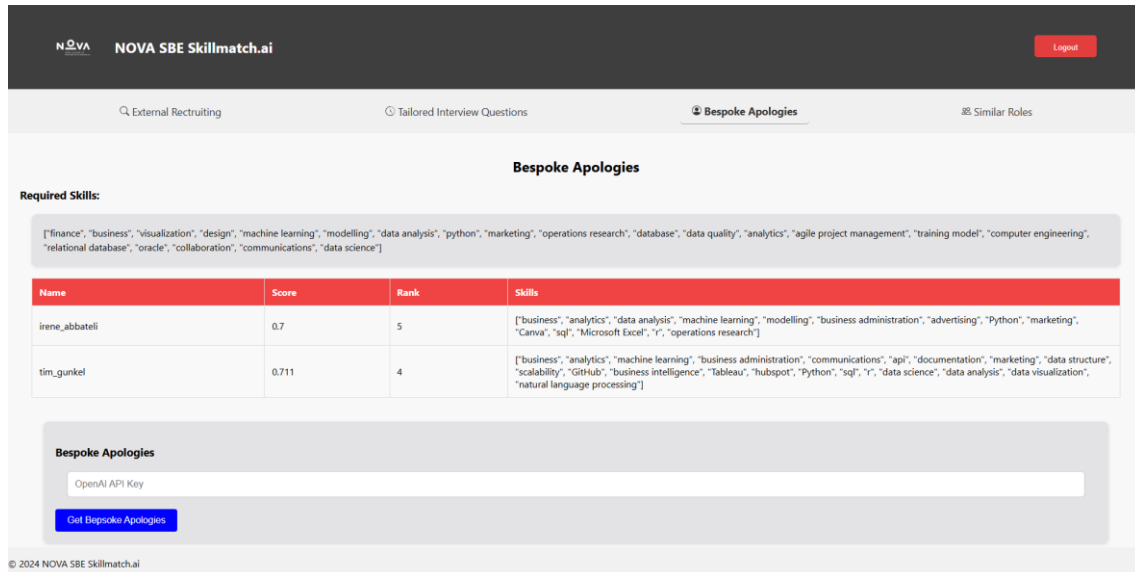
Figure 69: The bespoke apologies endpoint before generating the bespoke apologies. The Required Skills list highlights all the required skills from the job description while the table shows the applicants that did not meet the requirements and the skills they possess. If the active user is the admin user, there is no need to input the OpenAI API key. Otherwise, the user should input their API key before generating the bespoke apologies.
