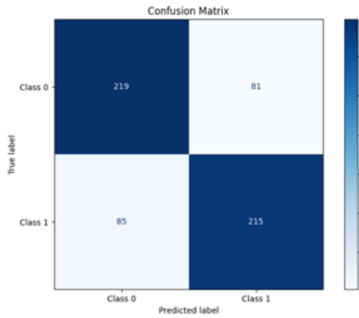
Figure 44: Confusion-Matrix - Threshold 0.5
