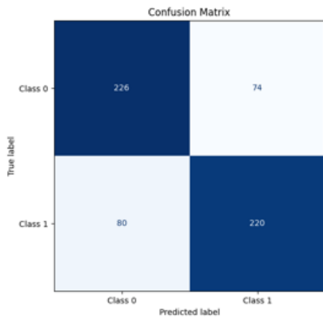
Figure 59: Confusion-Matrix - Cross-Encoder
