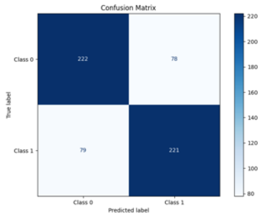
Figure 46: Confusion-Matrix - Threshold 0.6
