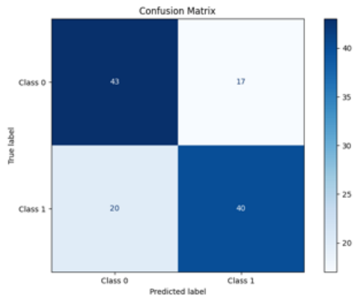
Figure 50: all-MiniLM-L6-v2- Confusion-Matrix
