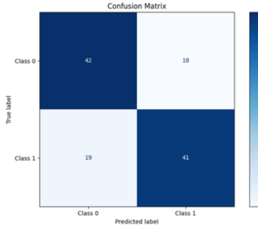
Figure 52: NV-Embed-v2 - Confusion-Matrix
