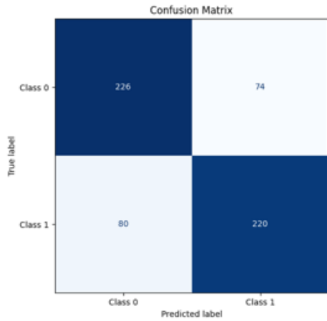
Figure 57: Confusion-Matrix - Bi-Encoder
