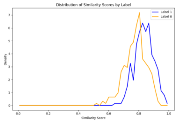
Figure 41: Distribution of Similarity Score by Labels - Threshold 0.3
