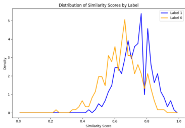
Figure 47: Distribution of Similarity Score by Labels - Threshold 0.6
