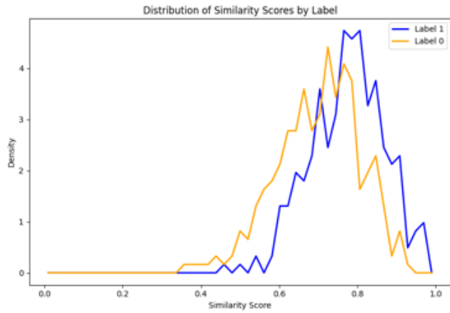
Figure 45: Distribution of Similarity Score by Labels - Threshold 0.5
