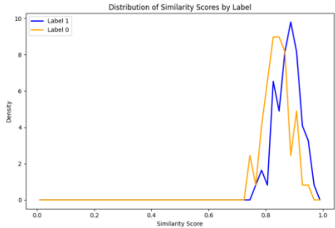
Figure 53: NV-Embed-v2 - Distribution of Similarity Score by Labels
