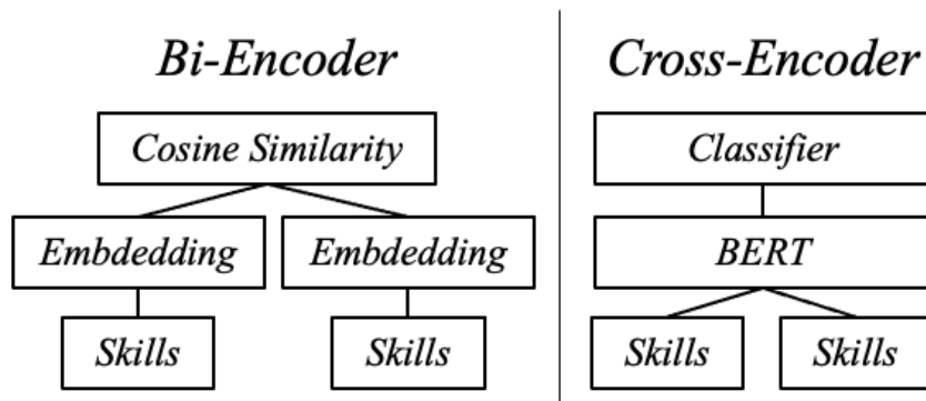
Figure 9: Encoder Architectures: Comparing Bi-Encoder Architecture with Cross-Encoder Architecture
