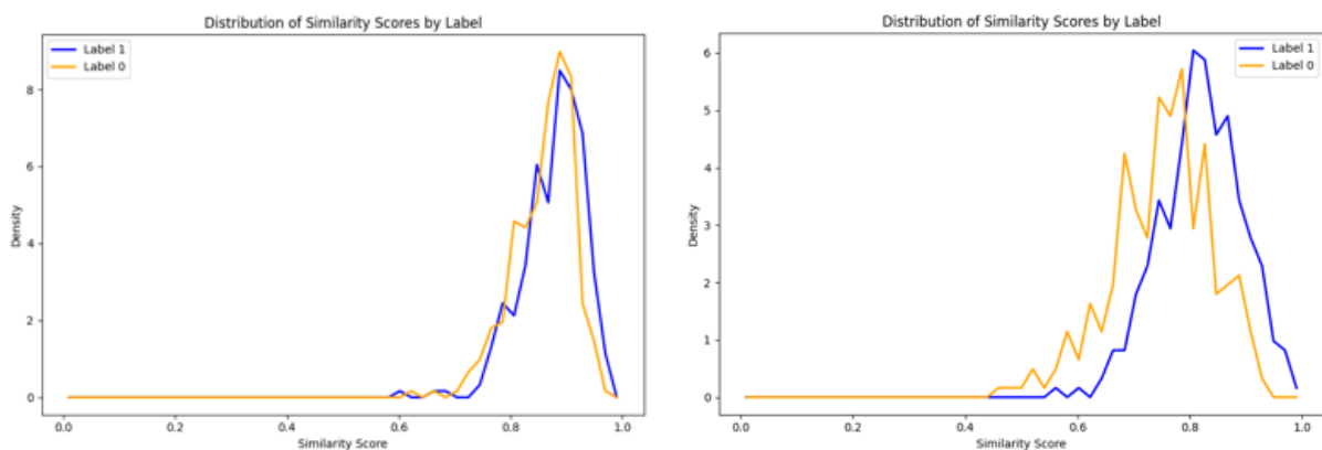
Figure 10: Distribution of Similarity Scores for Skill Representation Formats: This figure compares the similarity score distributions for Bag-of-Skills (left) and Skill-by-Skill (right). It shows that the Skill-by-Skill approach produces a clearer separation of scores between good-fit (Label 1) and bad-fit (Label 0) résumés.
