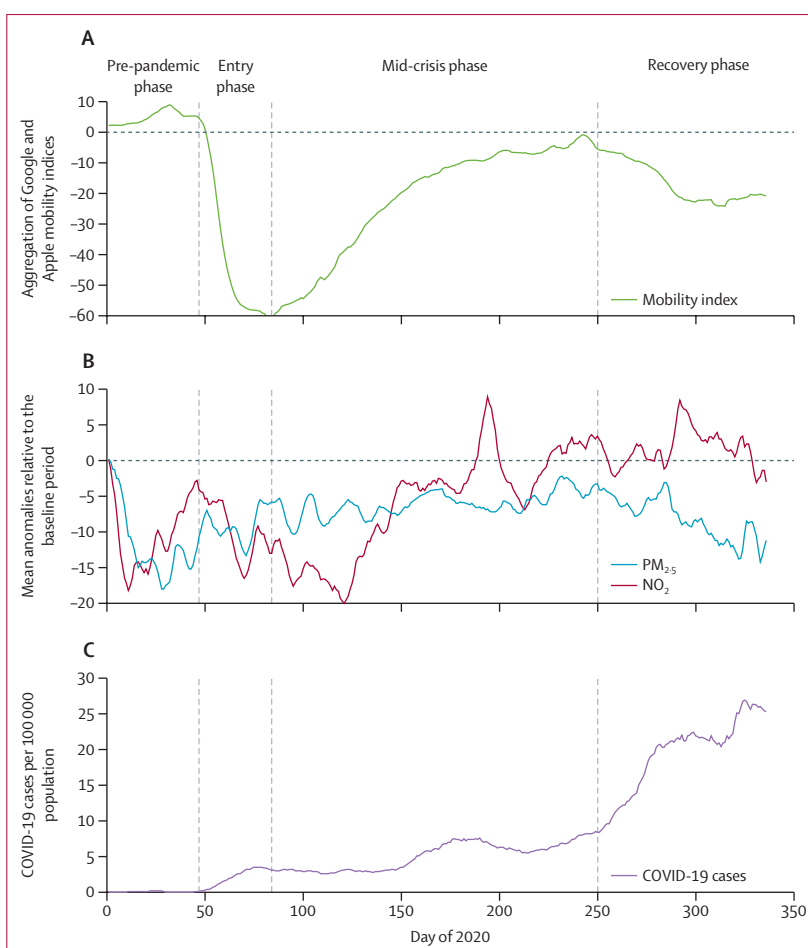
Figure 3: Overview of the progression of the COVID-19 crisis across 507 global cities in 2020
