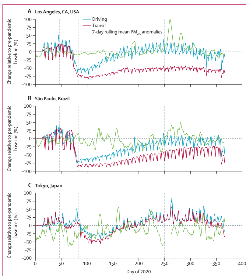
Figure 6: An overview of the relative shifts in transportation mode preferences (daily Apple mobility indices for driving and transit modes) and 7-day rolling mean PM 2.5 anomalies over 2020 for Los Angeles, CA, USA (A), São Paulo, Brazil (B), and Tokyo, Japan (C)
