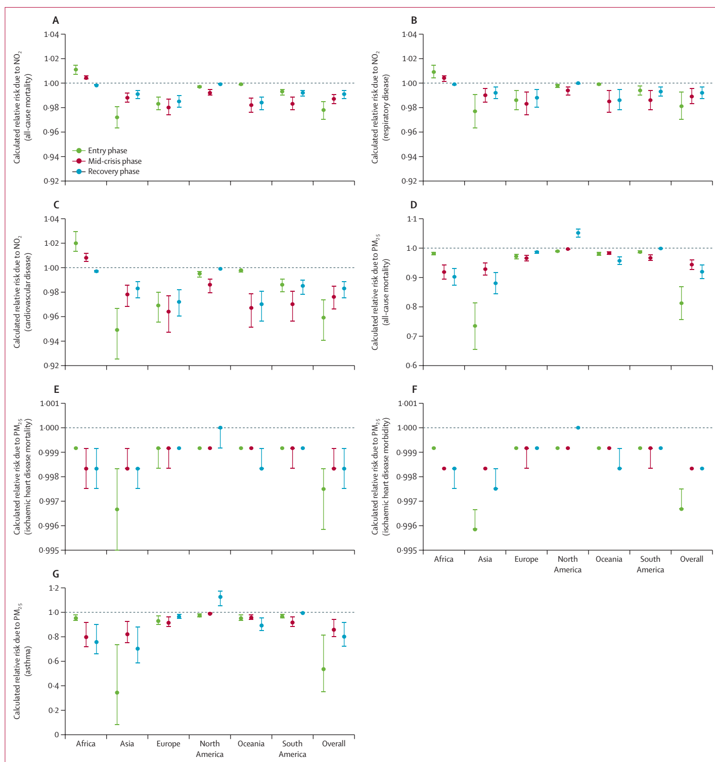
Figure 4: Relative health risks associated with air pollution reductions across continents and pandemic phases due to \text{NO}_2 (A–C) and \text{PM}_{2.5} (D–G)
