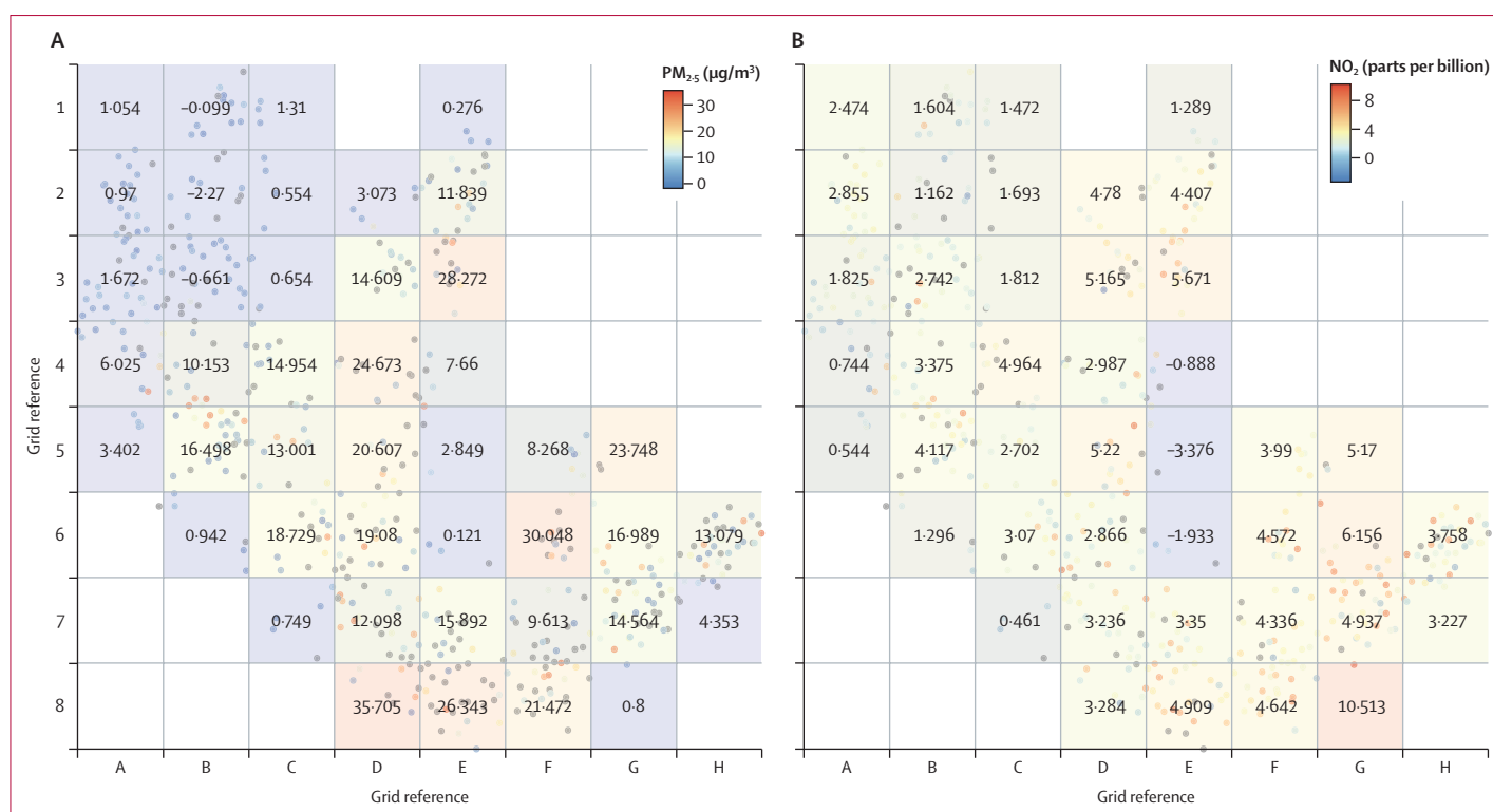
Figure 5: Mean anomalies of PM 2.5 (µg/m³; A) and NO 2 (parts per billion; B) across the period of days 84–250 in 2020 relative to the pre-pandemic baseline (ie, days 1–20 of 2020) for cities in each grid reference tile
