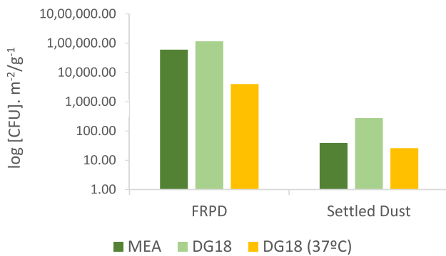
Fig. 2 Fungal counts obtained from used filter respiratory protective device (FRPD) (log [CFU]. m -2 ) and settled dust samples (log [CFU].g -1 ) inoculated in MEA and DG18 at 27 °C for environmental purposes and in DG18 at 37 °C for potential pathogenic evaluation
