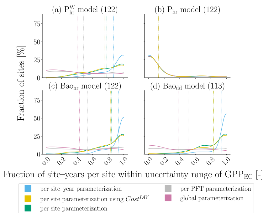
Figure 3. Distributions of fractions of site-years of a site for which annual average of simulated gross primary production ( GPP_{sim} ) was within the uncertainty range of eddy-covariance derived GPP ( GPP_{EC} ). The GPP_{sim} were estimated using (a) P-model of Mengoli et al. (2022) with drought stress, parameterized at hourly scale ( P_{hr}^W model), (b) P-model of Mengoli et al. (2022) without drought stress, parameterized at hourly scale ( P_{hr} model), (c) global best model of Bao, Wutzler, et al. (2022) parameterized at hourly scale ( Bao_{hr} model), and (d) global best model of Bao, Wutzler, et al. (2022) parameterized at daily scale ( Bao_{dd} model). Cost^{IAV} in the legend denotes the usage of an additional constraint on annual gross primary production flux during per-site parameterization. The dotted vertical lines represent the mean fractions of site-years of a site for which the annual average of GPP_{sim} was within the uncertainty range of GPP_{EC} . The mean values are summarized in Table E1. The numbers in parentheses beside the model name on top of each of the sub-figures represent the total number of sites. The model performance at an annual scale was calculated for fewer sites as some sites have a very low measurement period (Appendix C).
