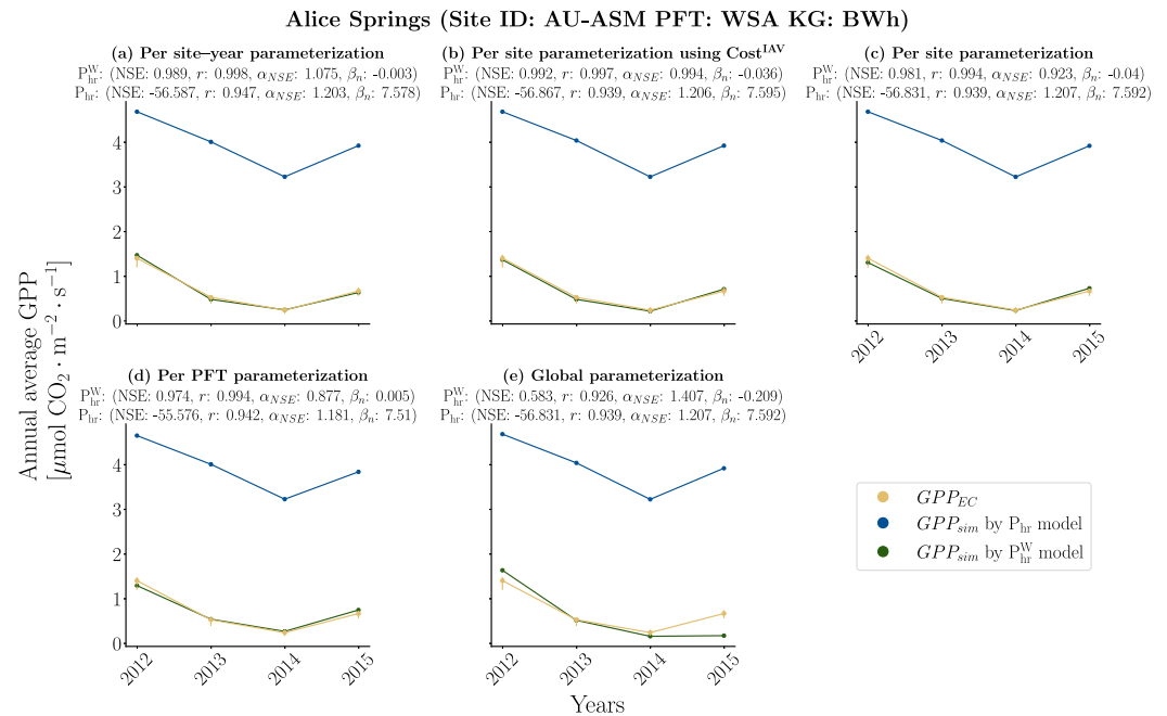
Figure 6. Comparison of annual average of gross primary production (GPP) derived by eddy covariance measurements ( GPP_{EC} ), and GPP simulated ( GPP_{sim} ) by the P-model of Mengoli et al. (2022) parameterized at hourly scale without drought stress ( P_{hr} model) and with drought stress ( P_{hr}^W model). The five subplots show simulated GPP from (a) site-year specific parameterization, (b) site-specific parameterization using an additional constraint on inter-annual variability in the cost function ( Cost^{AV} ), (c) site-specific parameterization, (d) plant-functional types (PFT) specific parameterization, and (e) global parameterization. The values of model performance measures (Nash-Sutcliffe efficiency, viz. NSE, correlation coefficient, viz. r , relative variability, viz. \alpha_{NSE} , and bias, viz. \beta_n ) are shown on top of respective subplots. This site is dominated by Mulga ( Acacia aneura ), and had an annual average temperature of \approx 22^\circ\text{C} , and an annual average precipitation of \approx 318 mm during the observation period (Cleverly et al., 2013; Pastorello et al., 2020). The vertical error bars represent the uncertainty range (see Section 2.4.3) of the annual average of GPP_{EC} for the corresponding years (the uncertainty range is relatively small for this specific site). The site ID, PFT, and Köppen-Geiger climate class (KG) of the site are provided on top of the figure in bold.
