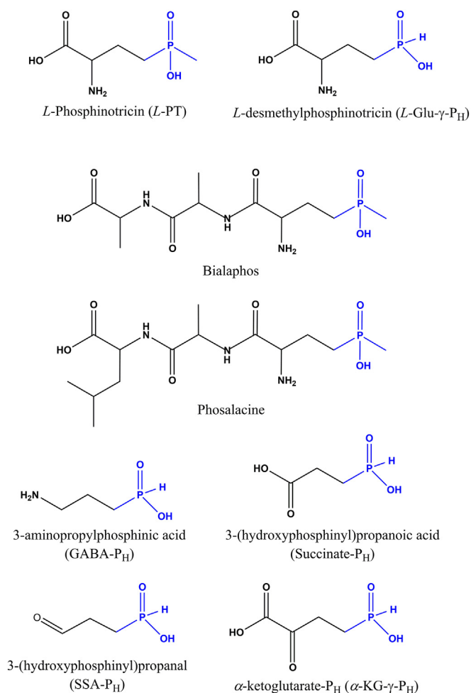
Figure 1. Structural formula of phosphinates. L-phosphinitricin (L-PT) and the natural tripeptides that derive from it (Bialaphos and Phosalacine) are shown along with the H-phosphinic compound L-Glu-γ-P H (L-desmethylphosphinitricin) and its derivatives obtained either by enzymatic decarboxylation (GABA-P H ), followed by transamination (SSA-P H ) and oxidation (succinate-P H ), or by either transamination or oxidative deamination (α-KG-γ-P H ).
