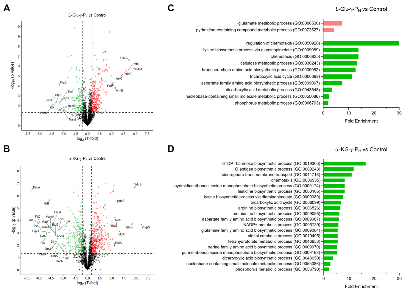
Figure 4. Volcano plots and Gene Ontology (GO) enrichment analyses. The graphs illustrate differentially abundant proteins and most affected pathways upon exposure to L-Glu-γ-P H or α-KG-γ-P H . A and B , Volcano plots of all proteins identified in the proteome database when cells were challenged with L-Glu-γ-P H ( A ) or α-KG-γ-P H ( B ). Green points: differentially expressed proteins that were significantly downregulated (T-fold < -1.5; p < 0.05). Red points: differentially expressed proteins that were significantly upregulated (T-fold > 1.5; p < 0.05). Proteins whose T-fold is > 8 or < -8 are text-labelled. C and D , Bar charts showing the GO terms for biological process ranked by fold enrichment of cells exposed to L-Glu-γ-P H ( C ) or α-KG-γ-P H ( D ). Green bars: significant downregulated pathways ( p < 0.05). Red bars: significant upregulated pathways ( p < 0.05).
