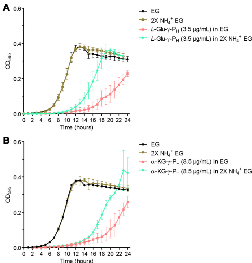
Figure 7. The increment in NH 4 + in EG medium improves the fitness of the cells when exposed to L -Glu-γ-P H and α-KG-γ-P H . At sub-inhibitory concentrations, L -Glu-γ-P H (3.5 μg/mL; A) and α-KG-γ-P H (8.5 μg/mL; B) delay cell growth in EG medium pH 7.0 (red squares) compared to the untreated group (black dots). In the same experimental conditions, a 2-fold increase in the ammonium content (2X NH 4 + EG) mitigates the inhibitory effect of L -Glu-γ-P H (A) and α-KG-γ-P H (B) on cell growth (green rhombus) compared to the untreated group (brown dots). No significant NH 4 + -related effect is observed if the untreated cells are grown in 2X NH 4 + EG (brown dots) compared to EG (black dots). Data, shown as mean ± sd, are the averages of at least three independent experiments.
