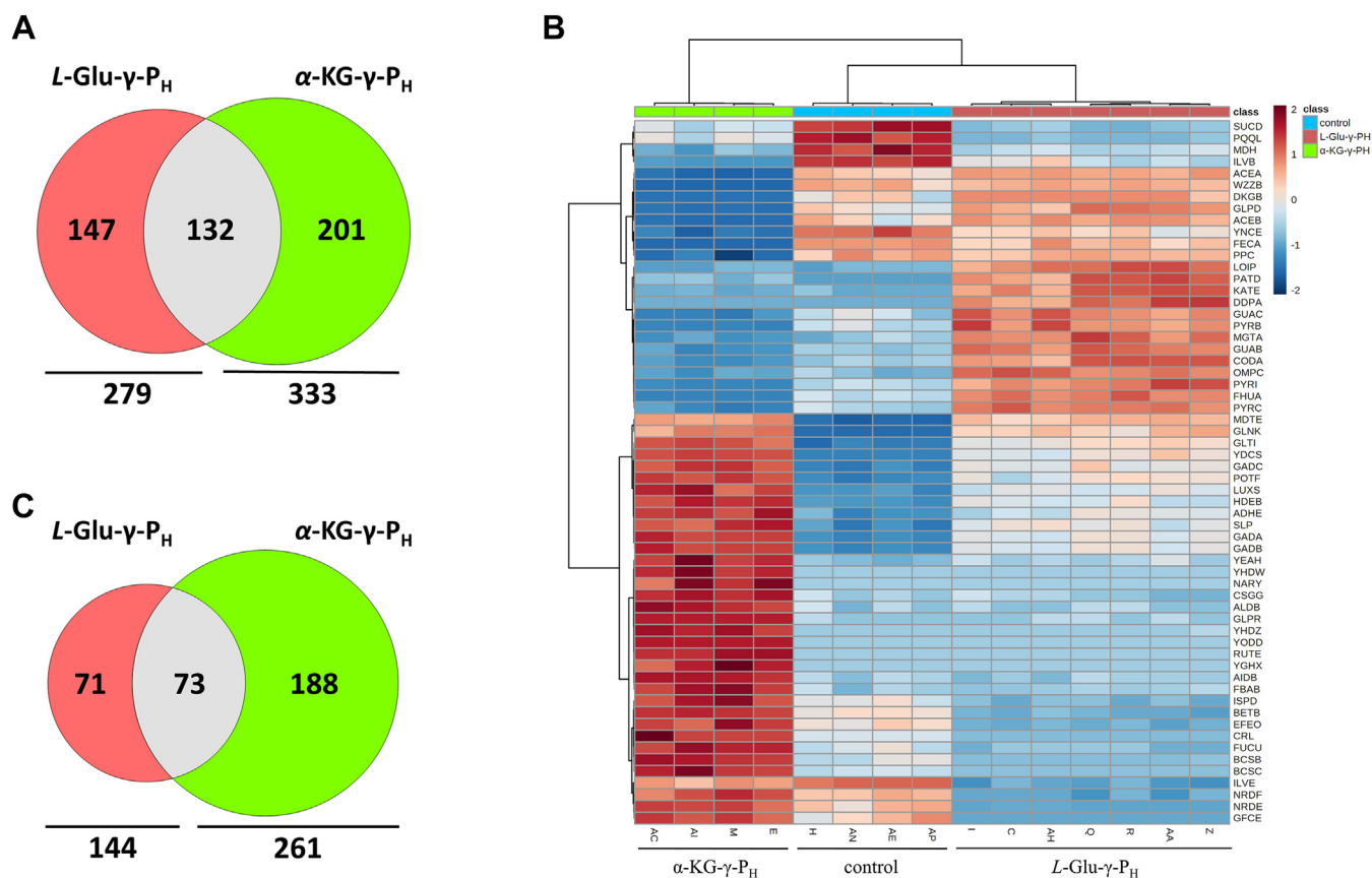
Figure 5. Venn diagrams and Heatmap visualization illustrate differentially abundant proteins upon exposure to L-Glu-γ-P H or α-KG-γ-P H . A and B, values in the Venn diagrams indicate the number of proteins that were upregulated (A) or downregulated (B) when cells were treated with L-Glu-γ-P H or α-KG-γ-P H . Numbers in the overlapping circles refer to proteins that were found to be co-upregulated (A) or co-downregulated (B) by both compounds. C, Heatmap visualization for the top 60 proteins based on the analysis of variance (ANOVA) test. Biological replicates (horizontal axis) and single proteins (vertical axis) are separated using a hierarchical clustering based on Euclidean distance.
