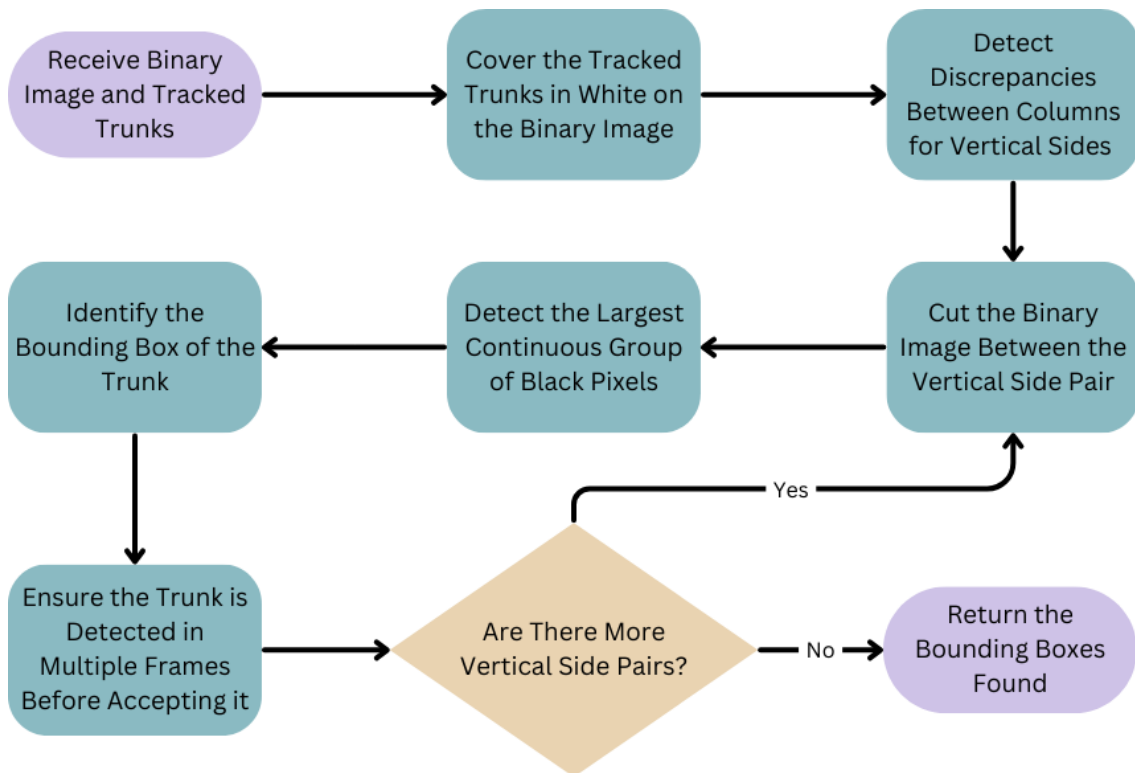
Figure 3.4: Flowchart of the New Trunk Detection process.
