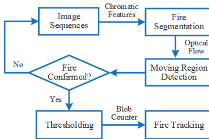
Figure 2.3: Flowchart of fire detection algorithms of paper Yuan, Liu, and Zhang 2016.
