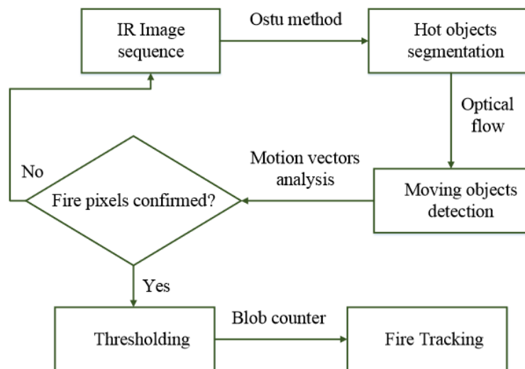
Figure 2.2: Illustration of the proposed fire detection algorithm of paper Yuan, Liu, and Zhang 2017.
