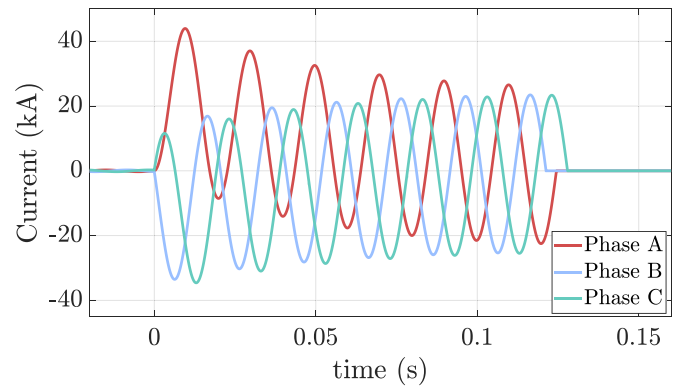
Figure 18. Simulated fault sequence alternating between normal operation and fault conditions.
