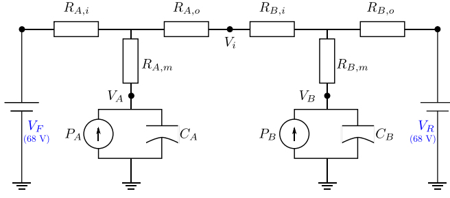
Figure 7. Mellor's thermal network for solution of the case example.
