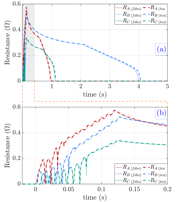
Figure 24. Comparison between the resistances calculated with fdm scheme and tea method for the three-phase concentric design: (a) the whole transient period and (b) only the first 200 ms.
