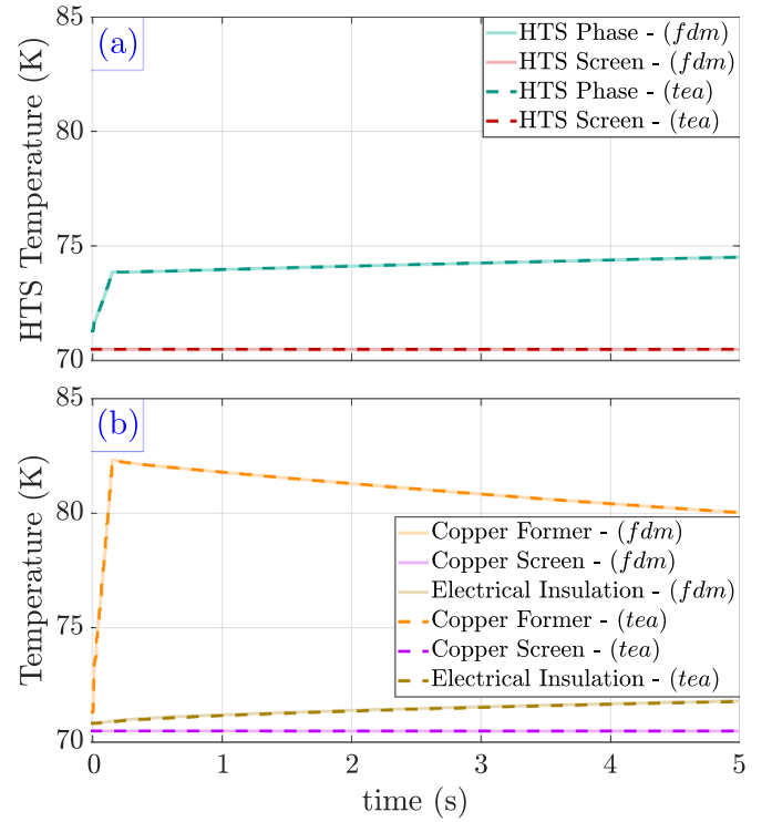
Figure 27. Comparison between temperature values at half cable length obtained with fdm scheme and tea method for the single-phase design. Temperature of (a) HTS layers and (b) electrical insulator, copper former and copper screen.
