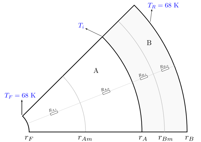
Figure 2. A sector-view of a hollow cylinder used for heat transfer analysis.
