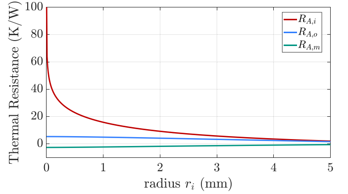
Figure 9. Behavior of the thermal resistance values when the internal radius tends to zero. Analysis for the full cylinder model.
