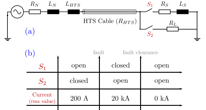
Figure 17. (a) Electrical grid configuration for transient simulation and (b) switching sequence of S_1 and S_2 .
