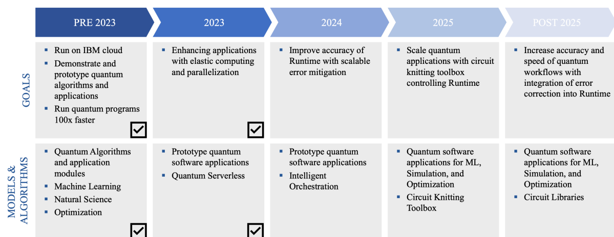
Figure 4: Quantum Roadmap
