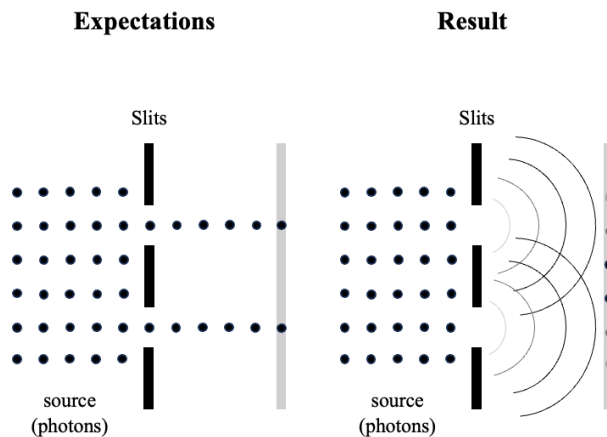
Figure 2: Double-Slit Experiment
