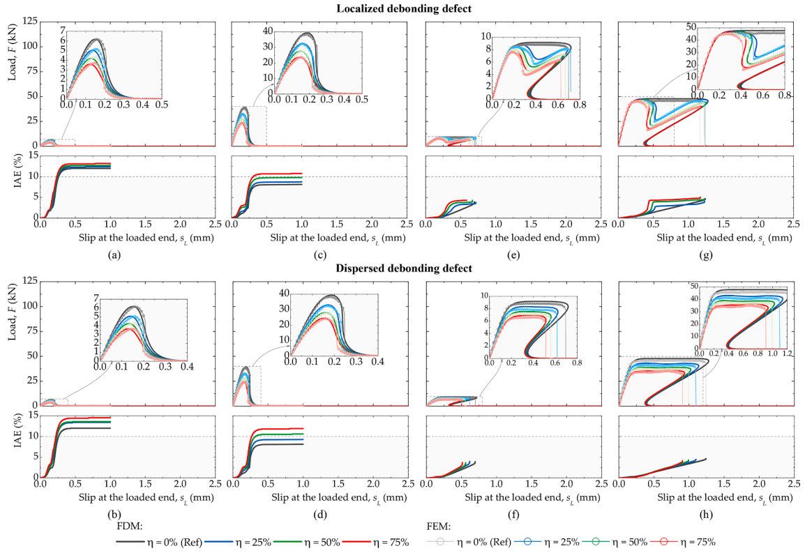
Fig. 9. Precision of the proposed FDM in the determination of the load vs. slip at the loaded end curves of the tests with a CFRP composite with a brittle adhesive and: (a)-(b) L_b = 50 mm; (c)-(d) L_b = 70 mm; (e)-(f) L_b = 200 mm; and (g)-(h) L_b = 350 mm.
