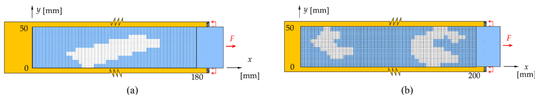
Fig. 12. Geometry of the debonding defects the specimens tested by Wang et al. [87] with a bonded length of: (a) 180 mm – A180-AD; (b) 200 mm – A200-AD.
