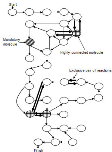
Fig. 1. Metabolic Network
