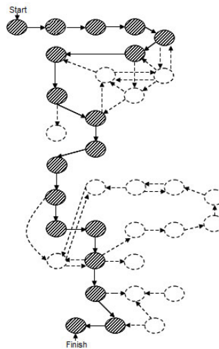
Fig. 2. Metabolic Pathway
