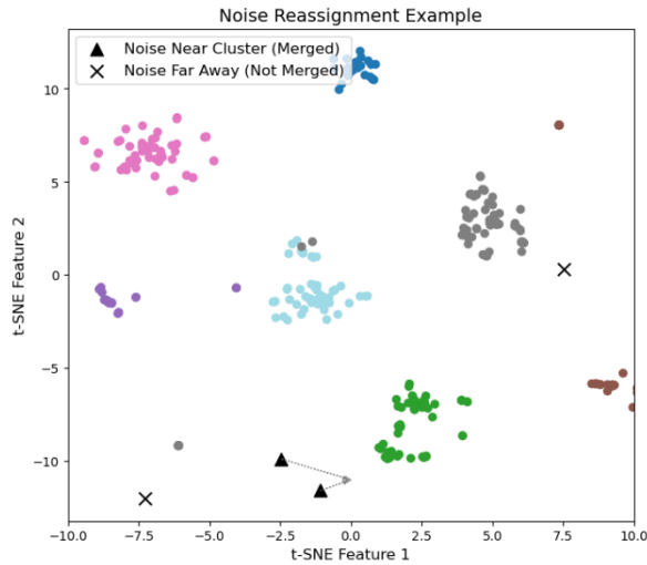
Figure D.4: How to handle noise.
