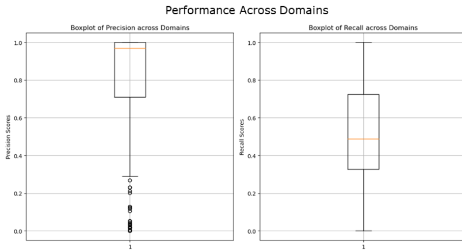
Figure D.7: Boxplots of performance metrics across different domains.
