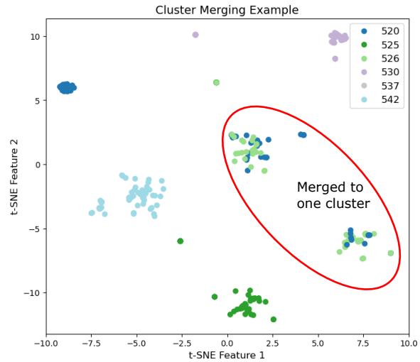
Figure D.5: How to merge clusters
