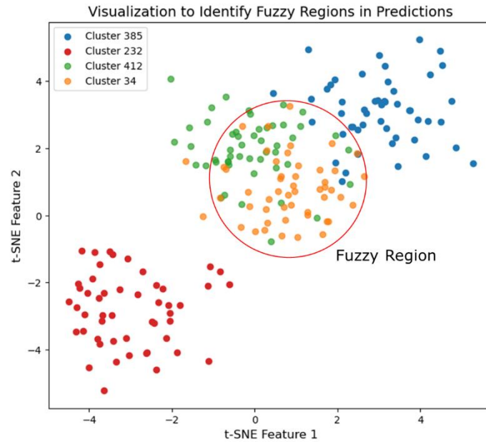
Figure D.9: Example of how clustering results can be visualized to identify fuzzy regions. Note that t-SNE is applied to embeddings, so fuzzy regions might sometimes also just be the reduced dimensions.
