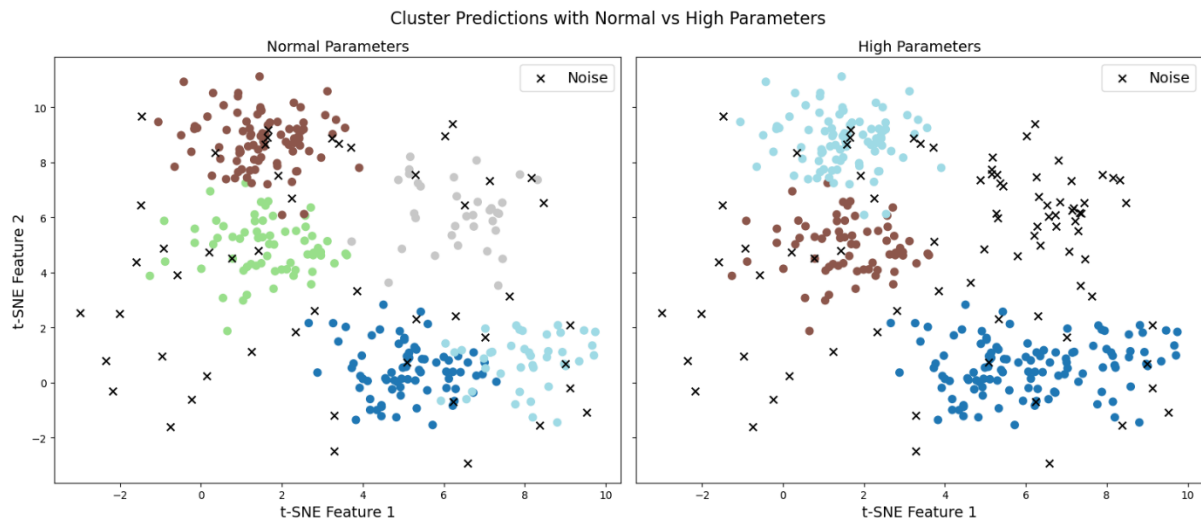
Figure D.8: Sample of cluster predictions with normal parameters and high parameters.
