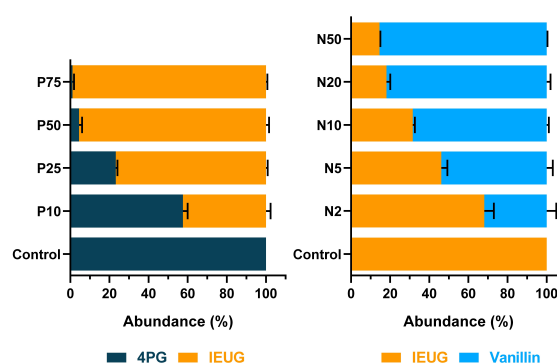
Figure 2. Conversions of 50 mM substrate of a) 4PG by P cells at different OD 600 values (10, 25, 50, and 75); and b) isoeugenol (IEUG) by N cells at different OD 600 values (2, 5, 10, 20, and 50). Reactions were performed in 50 mM KPi buffer, pH 7 in the presence of 10% (v/v) DMSO at 25 °C for 24 h. All experiments were performed in duplicate.
