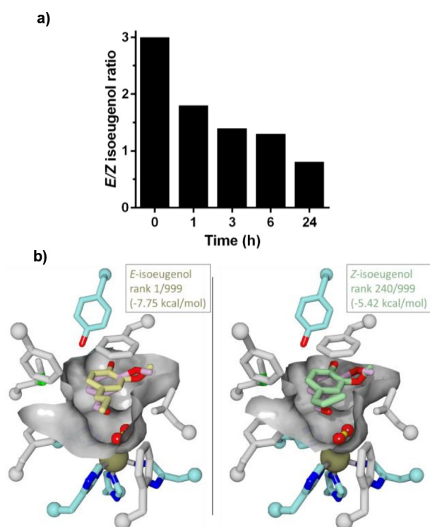
Figure 3. Substrate preference of NOV1 F . a) NMR analysis of the whole-cell conversion of 50 mM E/Z -isoeugenol (starting ratio E/Z = 75/25). N cells (OD 600 10) were used in 50 mM KPi buffer, pH 7, with 10% (v/v) DMSO as a cosolvent, at 25 °C; b) Docking result for NOV1 F with the E - (pale yellow left) and Z - (pale green, right) isomers of isoeugenol. Active site residues that were flexible during docking are white, frozen residues cyan, and the catalytic iron and oxygen are in gold and red, respectively. For comparison, the active site-bound vanillin from PDB:5J55 is shown in purple. While E -isoeugenol docked readily into the active site and with -7.75 kcal/mol binding energy is the highest ranking docking result out of 999 VINA runs, the Z -isomer docks mostly in non-catalytic positions (where the ligand's alcohol oxygen atom was more than 3.5 Å from the catalytic oxygen of Y101). The best (<3.5 Å O–O distance) catalytic pose of Z -isoeugenol binds with 5.42 kcal/mol as rank 240 – significantly less than the top-ranked (non-catalytic) pose, which binds with -7.17 kcal/mol.
