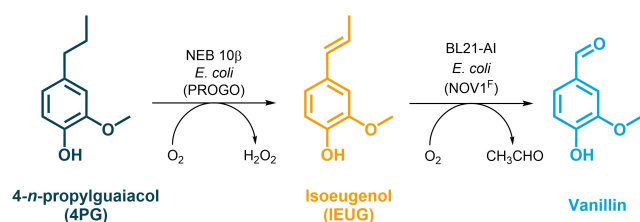
Scheme 1. The developed whole-cell cascade for vanillin production from 4PG.
