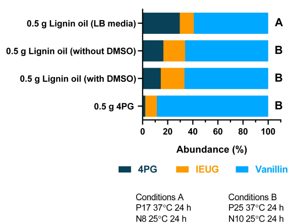
Figure 7. One-pot conversions of commercial 4PG and lignin-derived oils using a whole-cell, multi-enzyme cascade in a step-wise fashion under different experimental conditions. One-pot conversions of 0.5 g lignin oil or 4PG in KPi buffer (50 mM, pH 7). For conversions of 0.5 g lignin oil, the effect of 10% (v/v) DMSO as cosolvent was tested. To catalyse the first step of the process, P cells at OD_{600} 25, and N cells at OD_{600} 10 were used in the second step. A conversion of 0.5 g RCF oil was performed using P and N cells at OD_{600} 17 and OD_{600} 8, respectively, resuspended in the growth media, i.e. LB media. All the reactions were shaken at 150 rpm at 37 °C for 24 h, followed by the change to 25 °C for 24 h.
