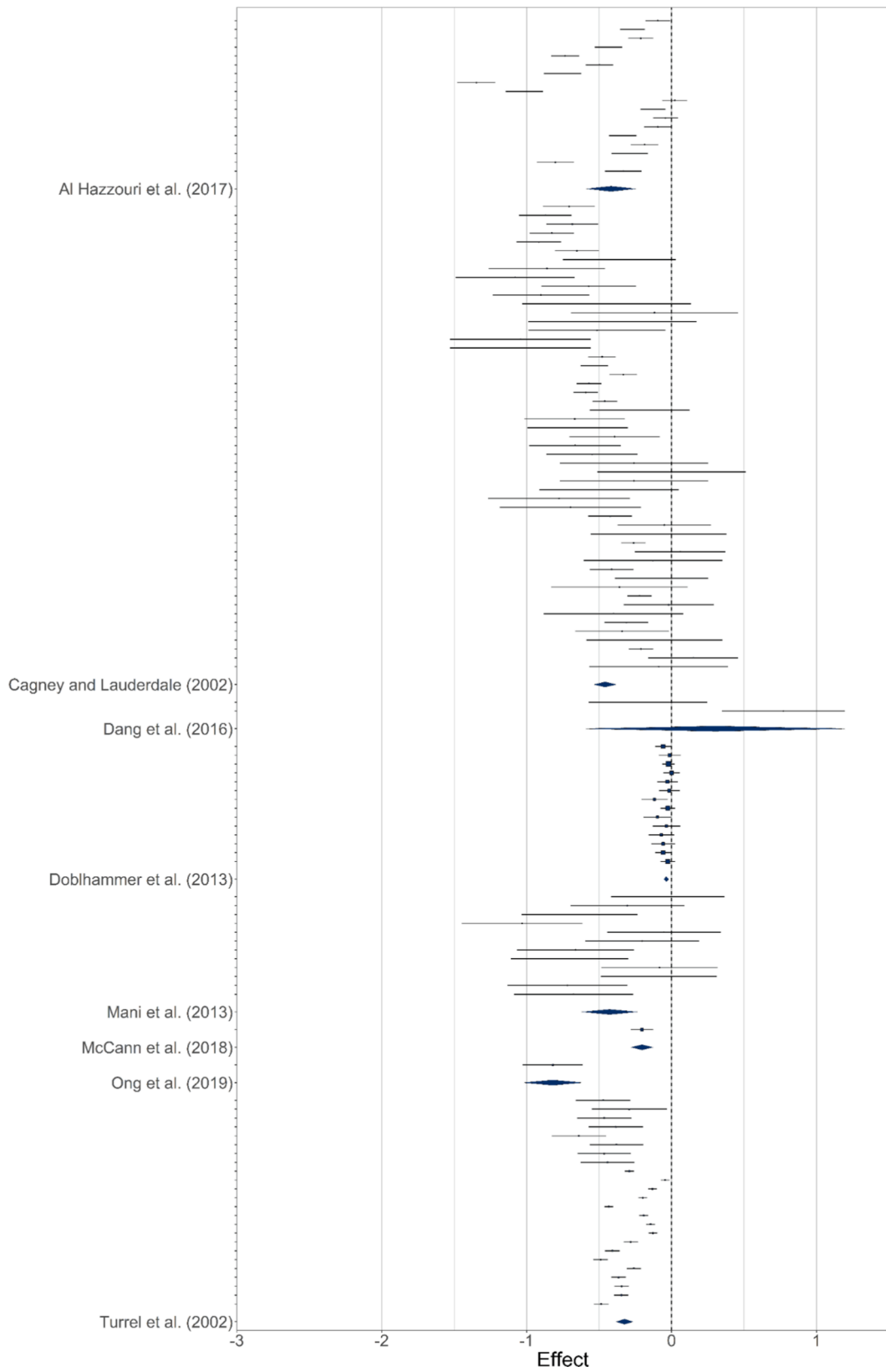
Fig. 1. Forest plot of effect sizes organized by study.
