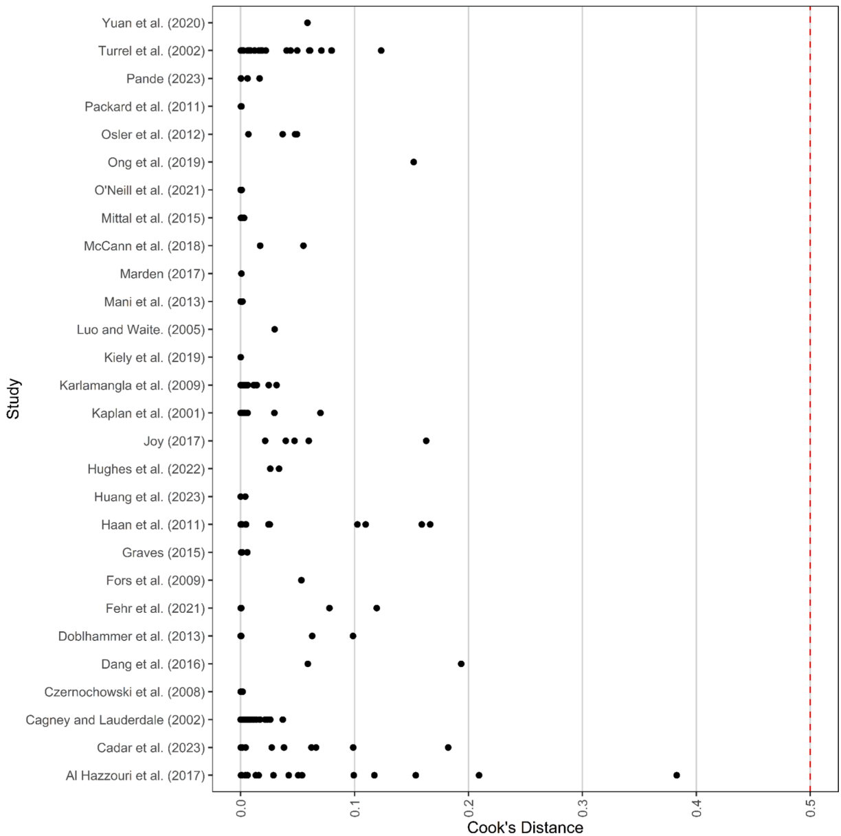
Fig. 2. Influence analysis results.
