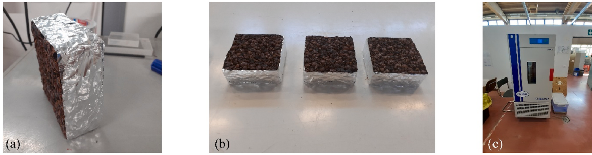
Fig. 5. (a) Detail of the aluminium foil used to provide a moisture barrier and expose only one surface of the sample to relative humidity variations; (b) three samples (10 cm × 10 cm × 4 cm) H1, H2, and H3, covered by the aluminium foil and considered to evaluate the hygroscopic properties; (c) climatic chamber (Climatest ARGOLab CH 250) employed for the hygroscopicity test.
