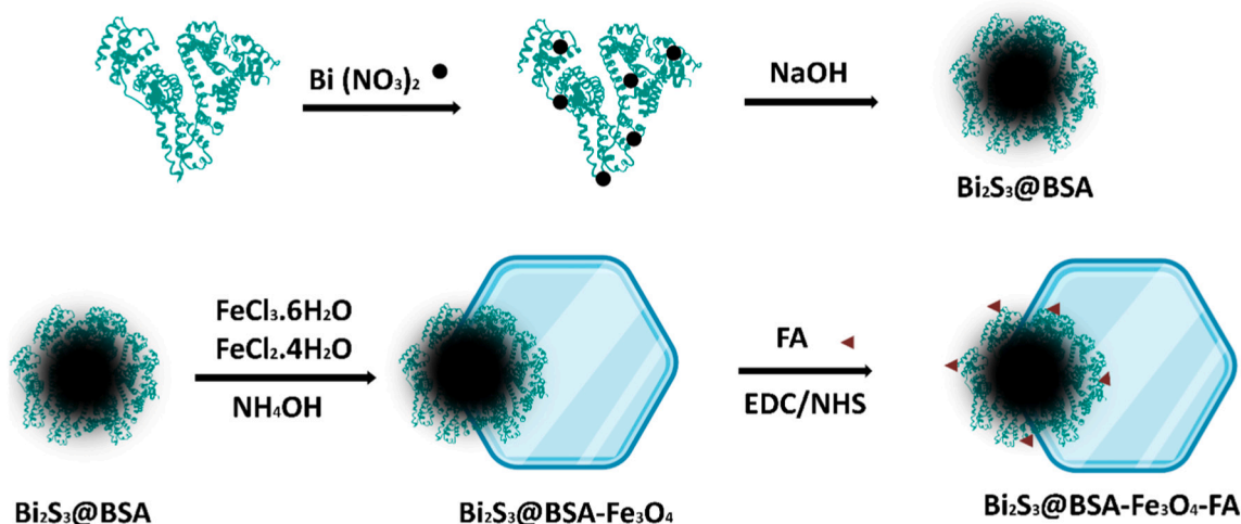
Fig. 1. (a) Schematic representation of the three steps in preparation of \text{Bi}_2\text{S}_3@BSA\text{-Fe}_3\text{O}_4\text{-FA} nanoradiosensitizers.
