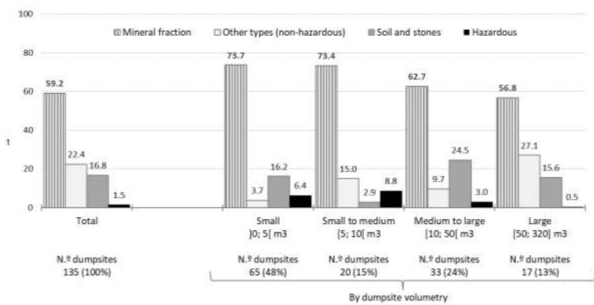
Figure 6.4 - Estimated physical composition for dumped construction and demolition waste, total and by dumpsite volumetry.
