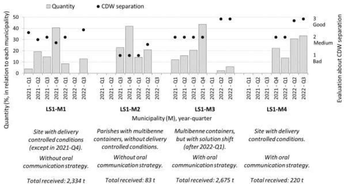
Legend: LS1 - Local Strategy 1 (Preliminary storage) Figure 7.2 - Municipal local solutions for construction and demolition waste preliminary storage.
