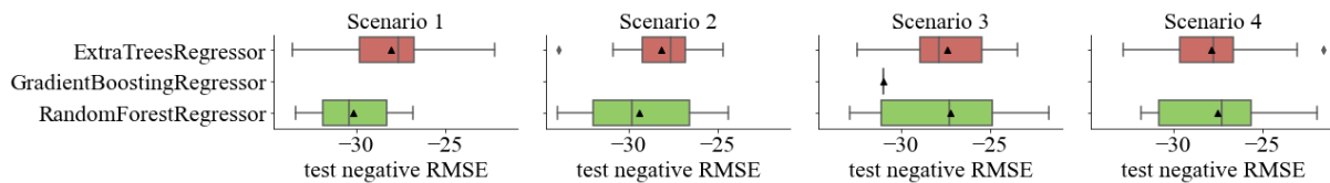
Figure 4.13 Test score distribution for each regressor of TPOT optimal pipelines for the bioavailability dataset.
