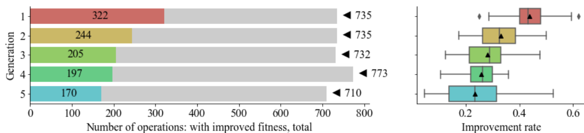
Figure 4.53 Amount and performance of mutations by generation. Bioavailability.
