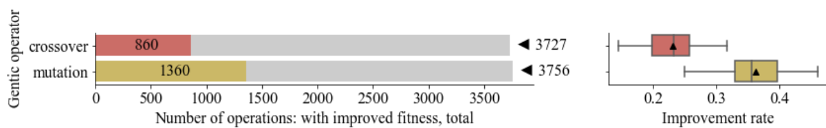
Figure 4.67 Amount and performance of operations by genetic operators. Concrete.
