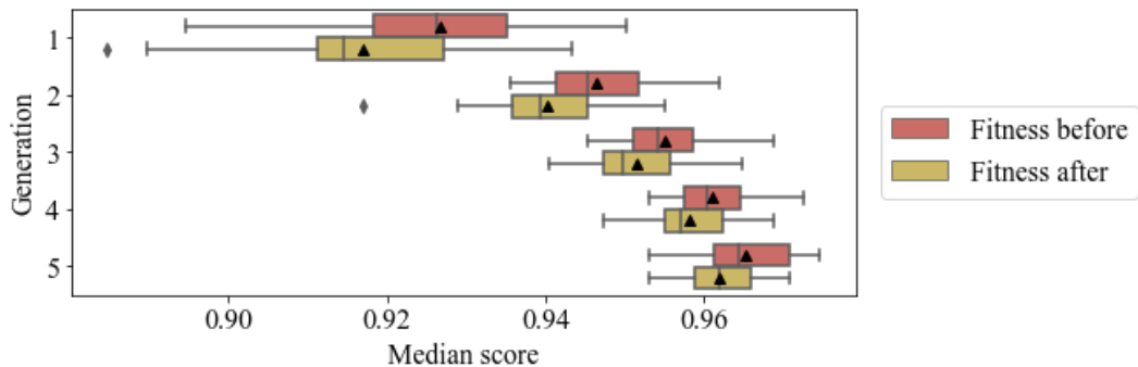
Figure 4.20 Distribution of median accuracies by the generation before and after genetic operation. Breast cancer.
