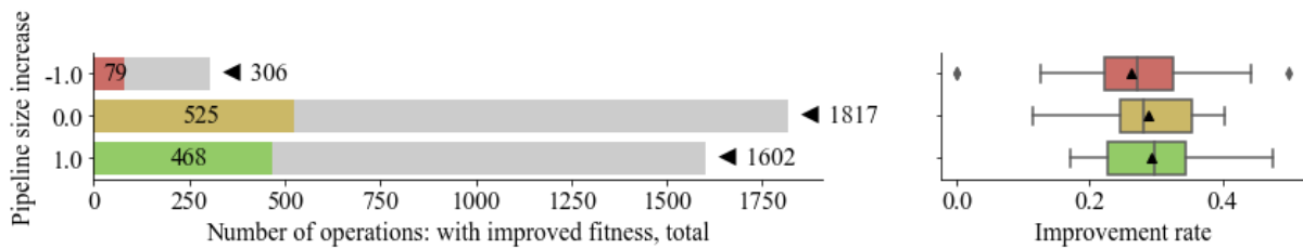
Figure 4.22 Amount and performance of mutations by pipeline size increase. Breast cancer.
