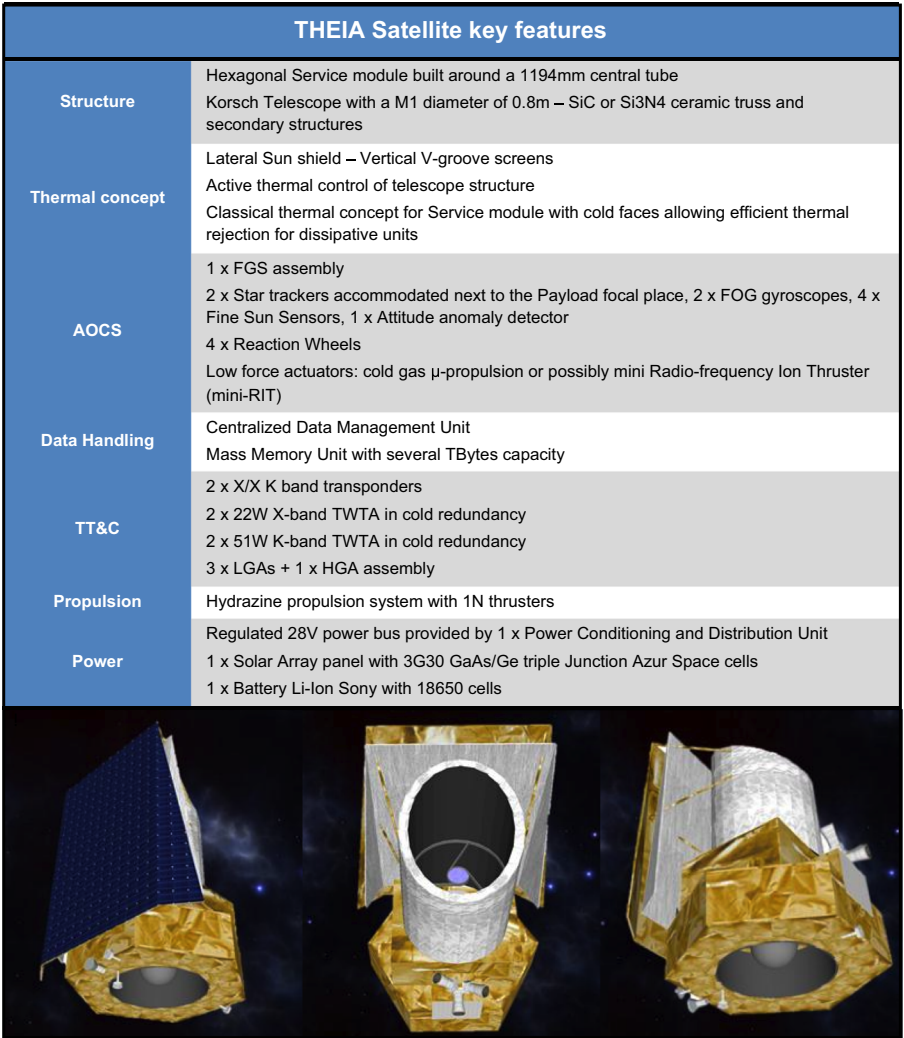
Fig. 21 Proposed Theia satellite concept (Thales Alenia Space). FGS: Fine Guidance Sensor; FOG: Fiber Optics Gyroscope; AOCS: Attitude and Orbit Control System,TT&C: Telemetry, Tracking & Control; TWTA: Travelling Wave Tube amplifier Assembly; LGA: Low Gain Antenna; HGA: High Gain Antenna
