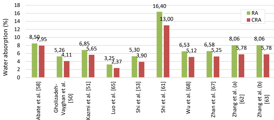
Figure 3. Water absorption of recycled aggregates before (RA) and after (CRA) being subjected to forced carbonation
