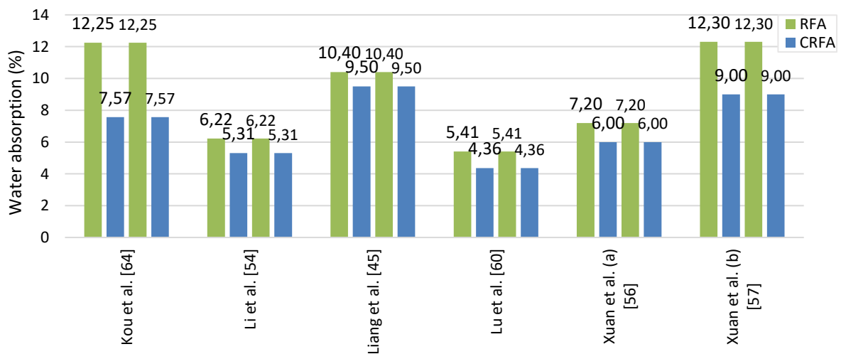
Figure 4. Water absorption of recycled fine aggregates before (RFA) and after (CRFA) being exposed to CO 2 curing
