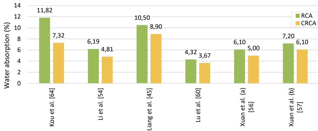
Figure 5. Water absorption of recycled coarse aggregates before (RCA) and after (CRCA) being exposed to CO 2 curing
