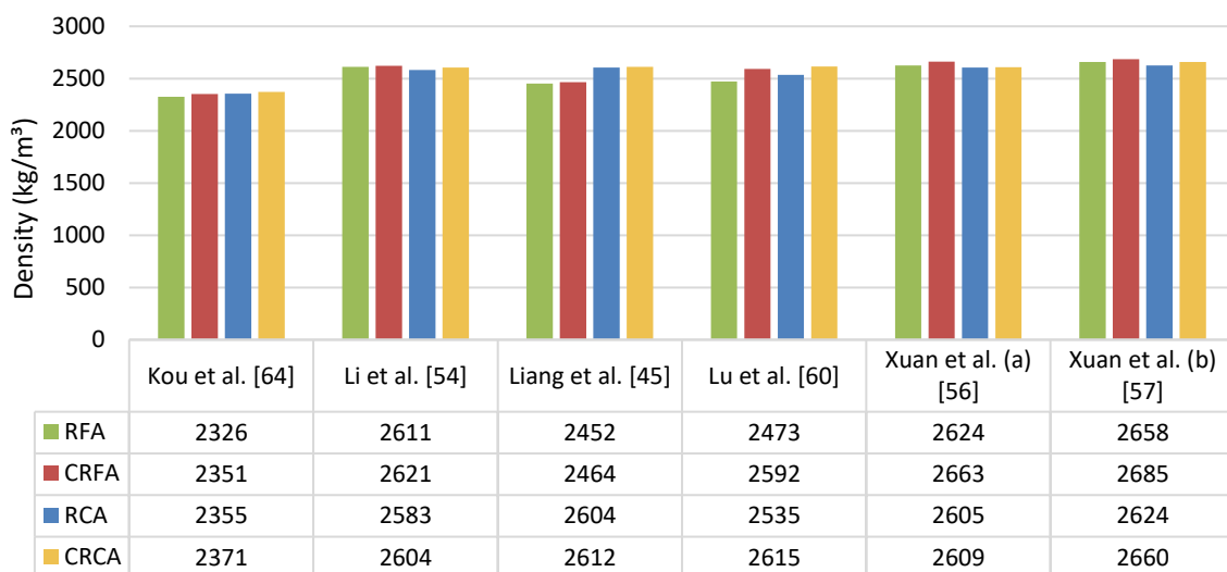
Figure 2. Bulk density of recycled fine aggregates (RFA) and recycled coarse aggregates (RCA) before and after subjected to forced carbonation (CRFA and CRCA)
