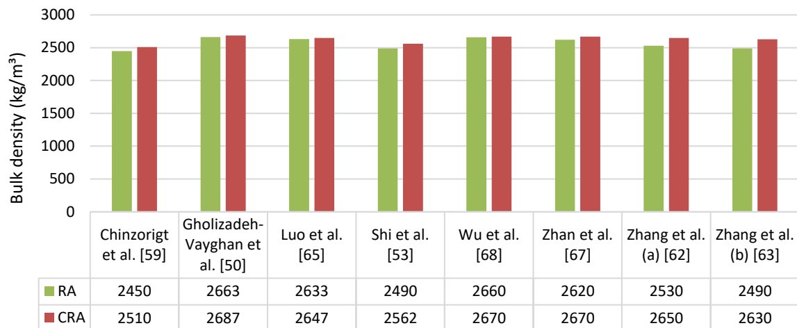
Figure 1. Bulk density of recycled aggregates before (RA) and after being exposed to CO 2 curing (CRA)
