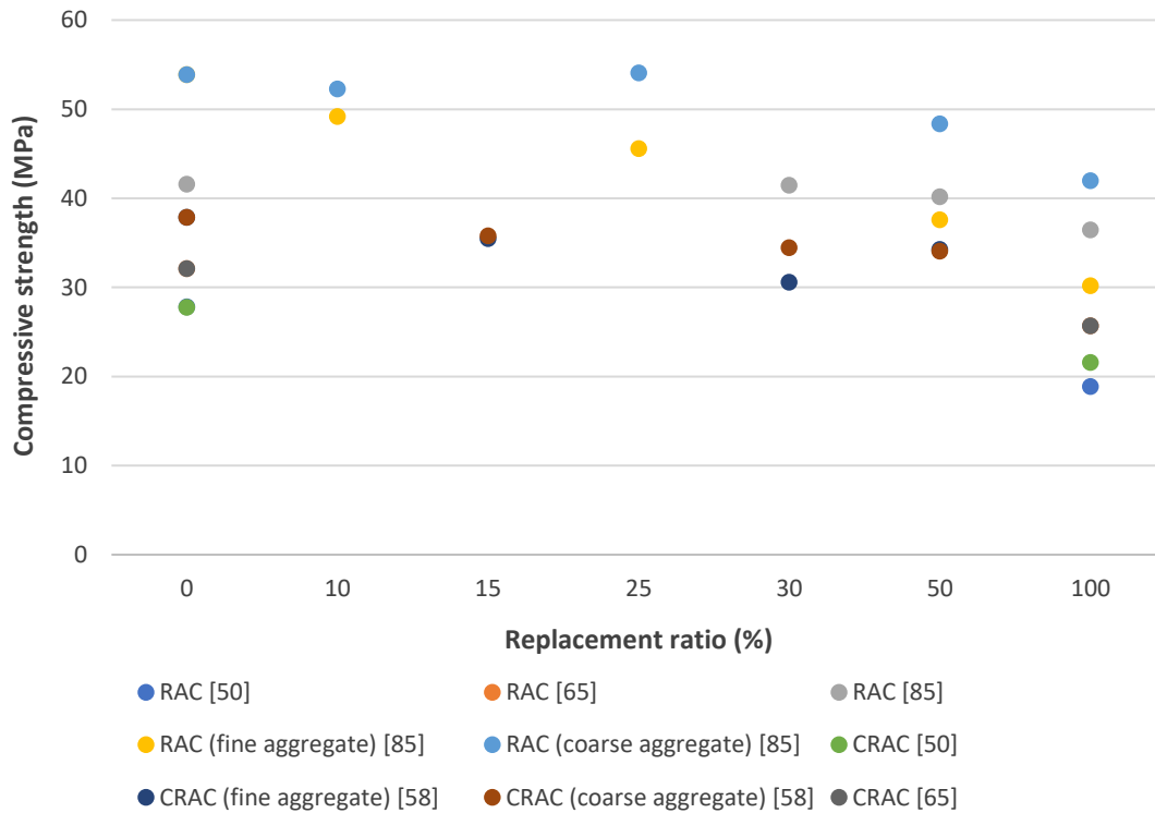
Figure 6. 28-day compressive strength of concrete containing recycled aggregates (RAC) and carbonated recycled aggregates (CRAC)
