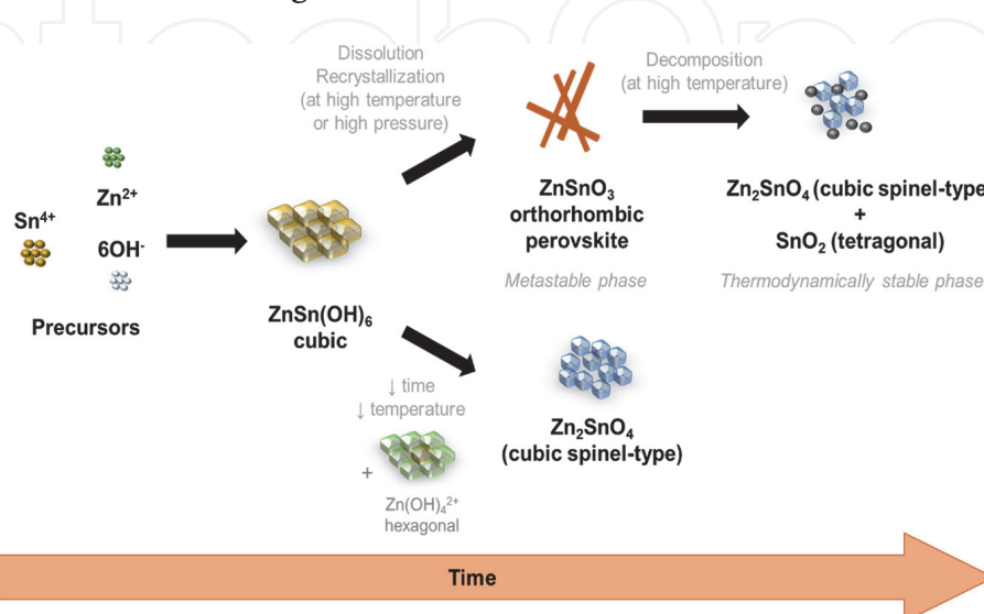
Figure 3. Schematic of the growth mechanism of ZTO nanostructures ( \text{ZnSnO}_3 nanowires and \text{Zn}_2\text{SnO}_4 nanoparticles) on a hydrothermal synthesis as a function of the energy available and the duration of the synthesis. From reference [43].
