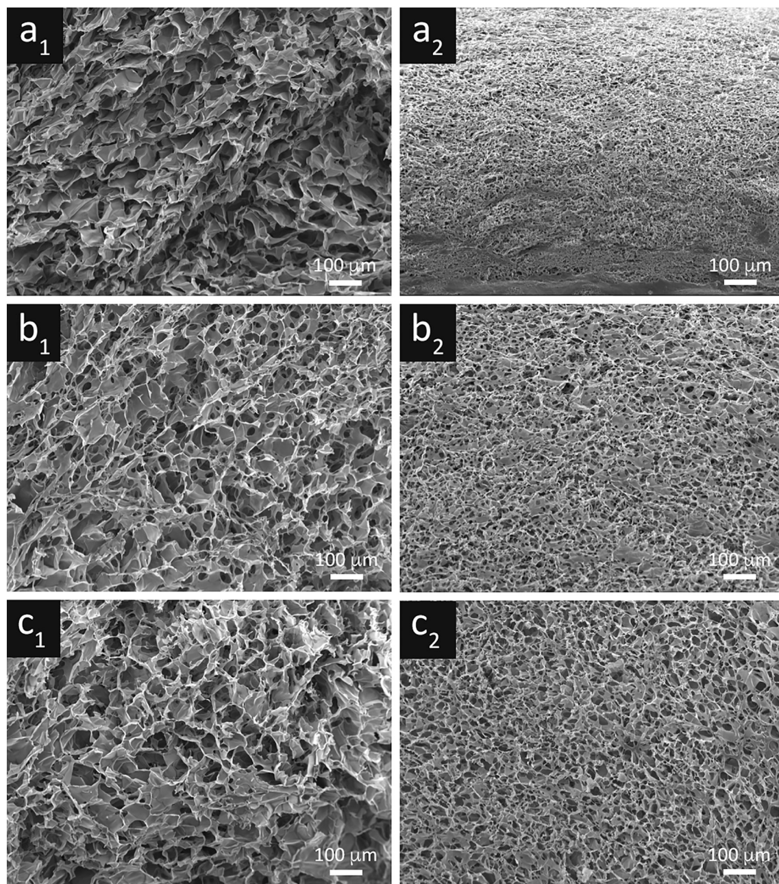
Fig. 2. SEM images showing the cutting section (1) and surface (2) of chitosan Oox-crosslinked scaffolds: CHT-1000x 45 (a), CHT-3000x 45 (b) and CHT-5000x 45 (c) (100× magnification).
