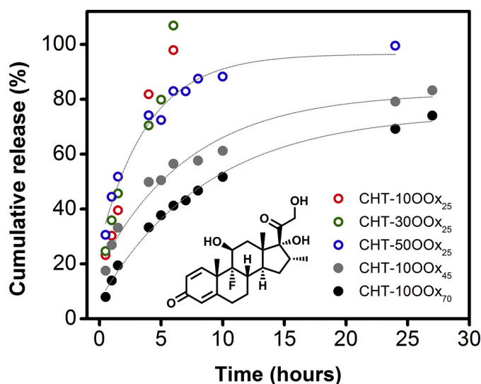
Fig. 6. Dexamethasone cumulative release from chitosan OOX-crosslinked scaffolds. Release profile from scaffolds with the same amount of crosslinker but different crosslinking rate and from scaffolds with different amount of crosslinker but the same crosslinking rate. The inset shows the chemical structure of dexamethasone.
