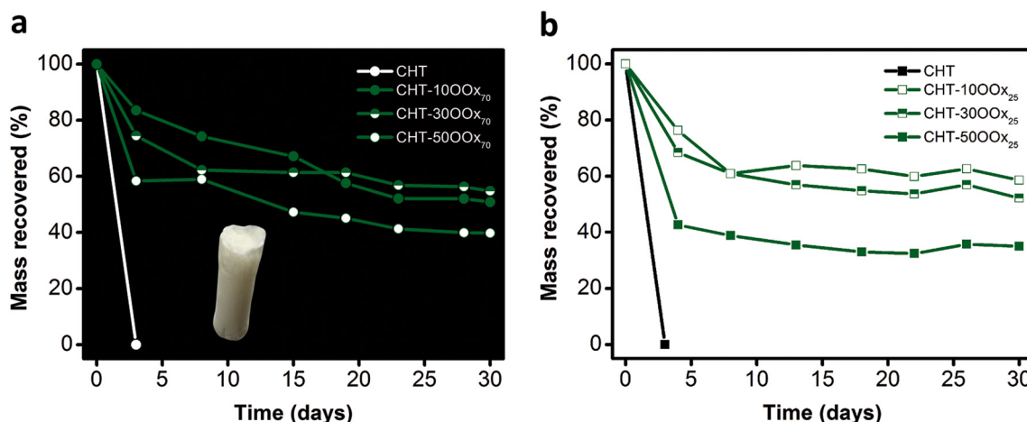
Fig. 4. Enzymatic degradation of chitosan Oox-crosslinked scaffolds using lysozyme at 37 °C for 30 days: CHT-100Ox 70 , CHT-300Ox 70 , CHT-500Ox 70 (a) and CHT-100Ox 25 , CHT-300Ox 25 , CHT-500Ox 25 (b). The inset picture shows a scaffold before the assay.
